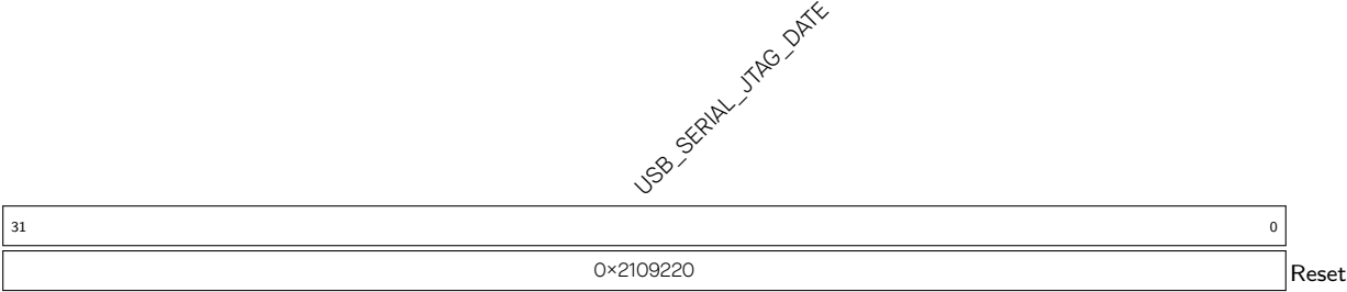
Register 30.28. USB_SERIAL_JTAG_DATE_REG (0×0080)
