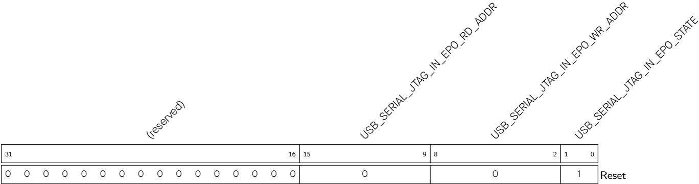
Register 30.18. USB_SERIAL_JTAG_IN_EPO_ST_REG (0×0028)
