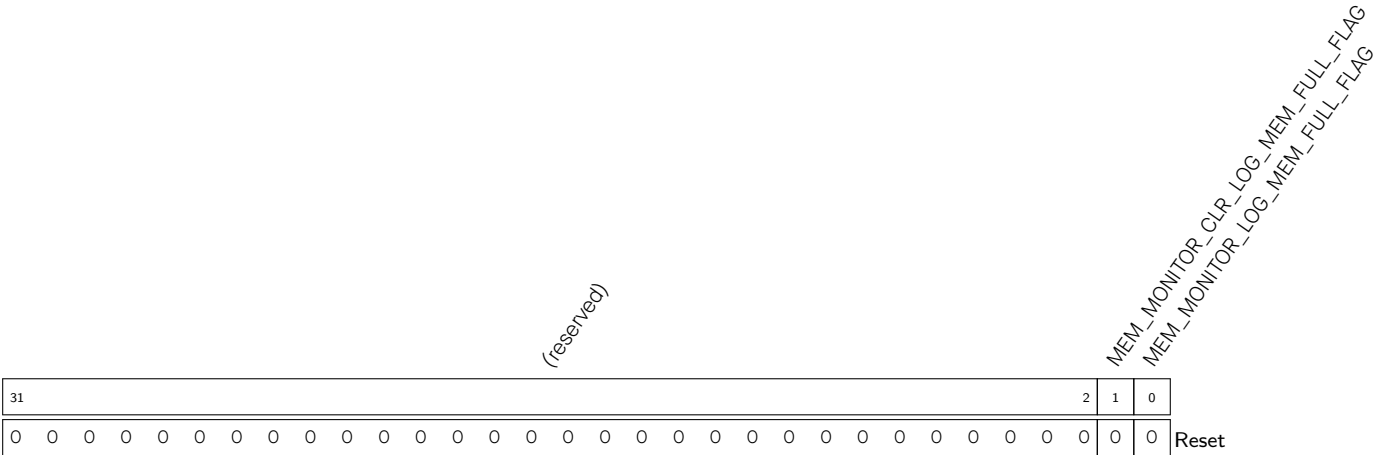
Register 16.10. MEM_MONITOR_LOG_MEM_FULL_FLAG_REG (0×0024)
