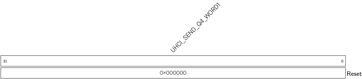
Register 25.53. UHCI_REG_Q4_WORD1_REG (0×0058)
