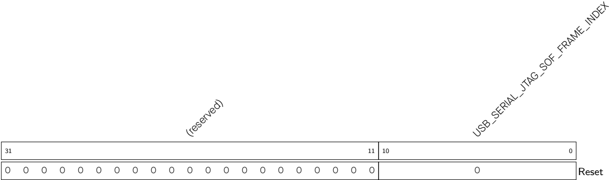
Register 30.17. USB_SERIAL_JTAG_FRAM_NUM_REG (0×0024)
