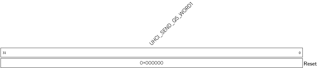
Register 25.55. UHCI_REG_Q5_WORD1_REG (0×0060)
