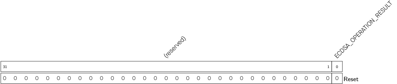
Register 23.9. ECDSA_RESULT_REG (0×0024)
