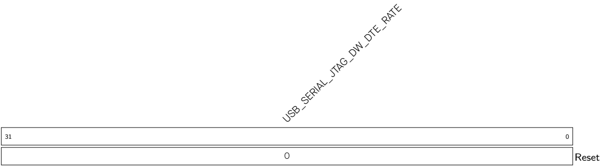
Register 30.25. USB_SERIAL_JTAG_SET_LINE_CODE_WO_REG (0×0050)
