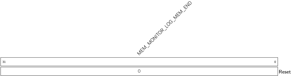
Register 16.7. MEM_MONITOR_LOG_MEM_END_REG (0×0018)
