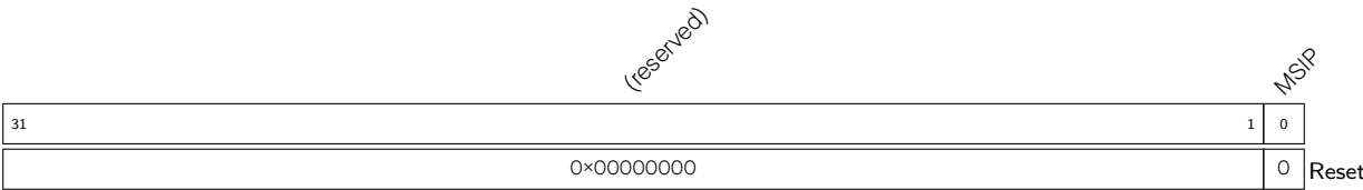
Register 1.25. MSIP (0×1800)
