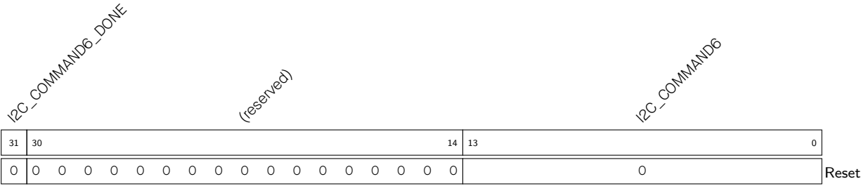
Register 27.31. I2C_COMD6_REG (0×0070)
