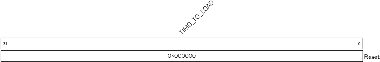
Register 12.9. TIMG_TOLOAD_REG (0×0020)
