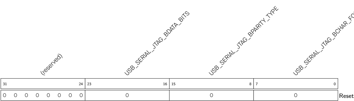
Register 30.26. USB_SERIAL_JTAG_SET_LINE_CODE_W1_REG (0×0054)
