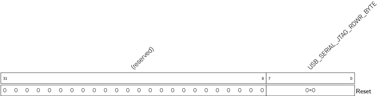
Register 30.1. USB_SERIAL_JTAG_EP1_REG (0×0000)
