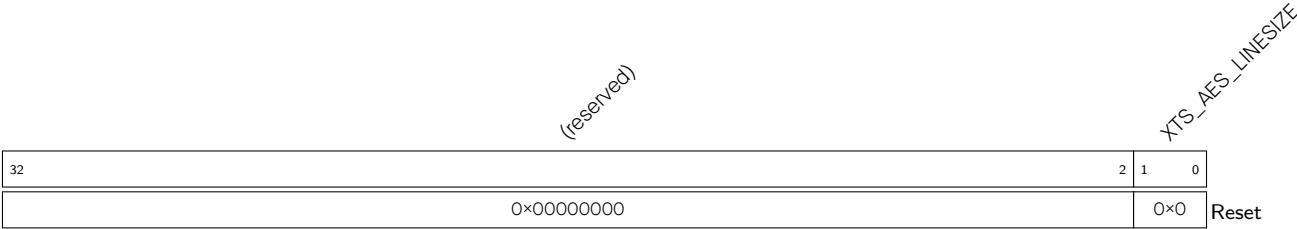
Register 24.2. XTS_AES_LINESIZE_REG (0×0340)
