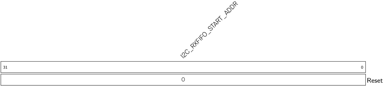
Register 27.35. I2C_RXFIFO_START_ADDR_REG (0×0180)
